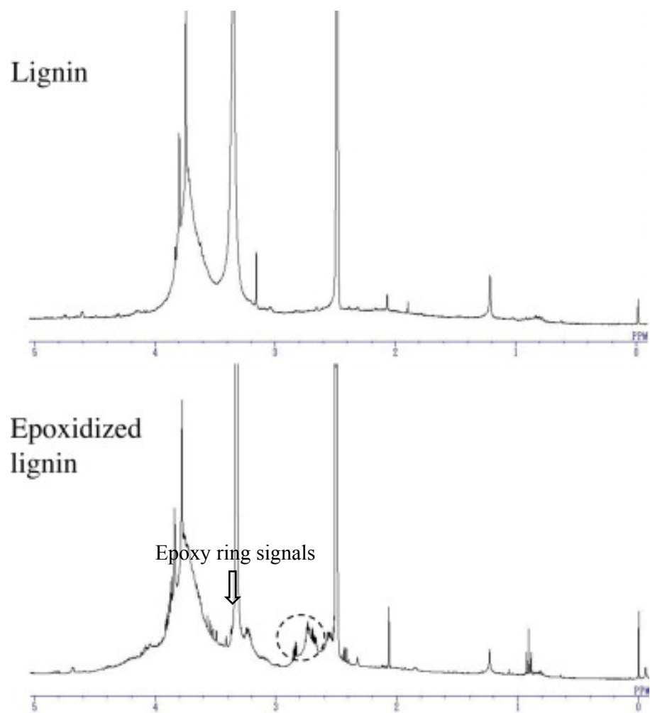
Figure 12: ^1\text{H} NMR Spectra of eucalyptus lignin and epoxidized eucalyptus lignin.
