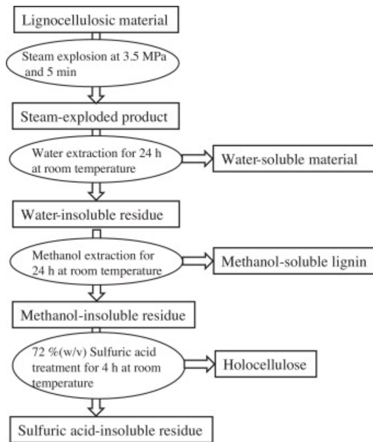
Figure 9: Extraction and separation procedure of lignocellulosic material.
