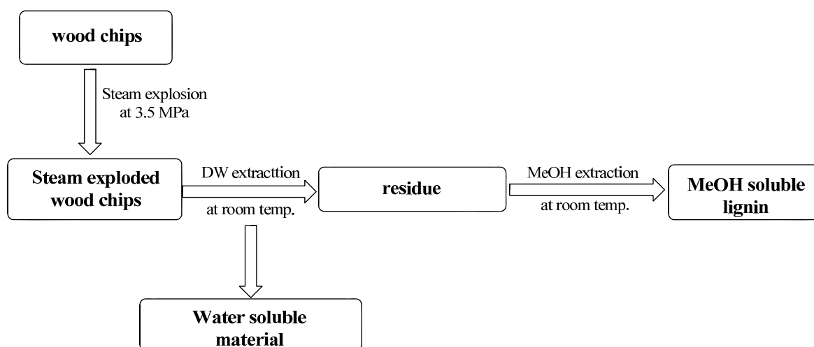
Figure 1: Extraction of lignin
