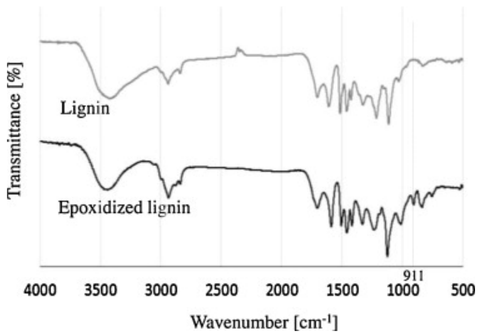
Figure 13: FT-IR spectra of eucalyptus lignin and epoxidized eucalyptus lignin.
